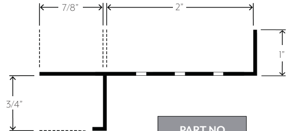
PART NO. WPM 75-V-200
