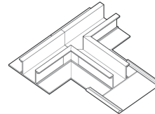
3 Way Tee Intersection (with Vinyl Connector)
