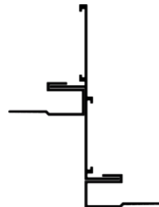
DRYWALL CEILING TRANSITION TO DRYWALL
