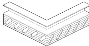
Outside Corner
